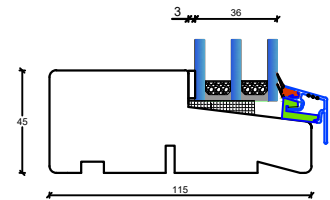
V4: Bundkarm faste partier
