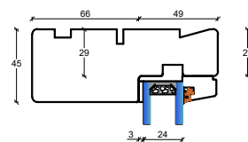
D6: Faste elementer, top karm
