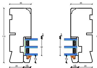
D5: Faste elementer, side karme
