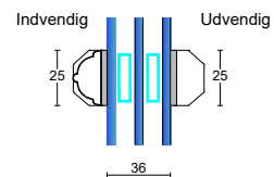
25 mm. energisprosse Modern
